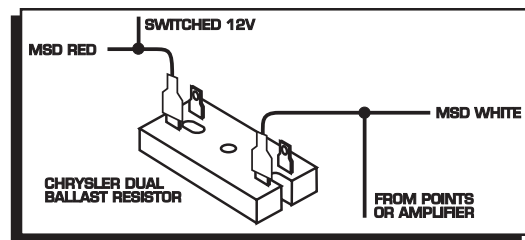
Figure 8 Wiring the Dual Ballast Resistor
