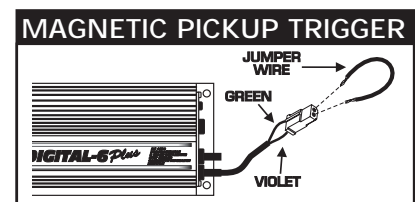
Figure 12 Checking for Spark with the Mag Pickup.
