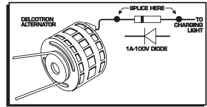
Figure 10 Installing the Diode to a 1973-1983 GM Vehicle.
