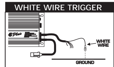
Figure 11 Checking for Spark with the White Wire.
