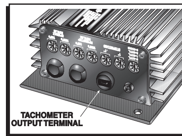
Figure 1 Tach Terminal
